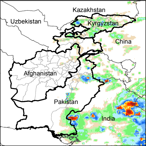
Daily Rainfall estimate for 5 Jul., 2017
