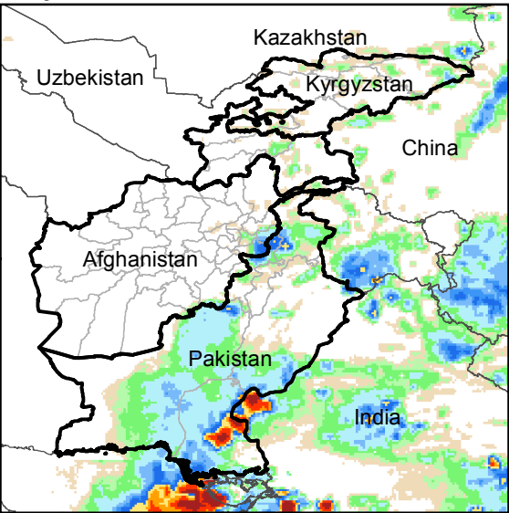
Daily Rainfall estimate for 19 Jul., 2017
