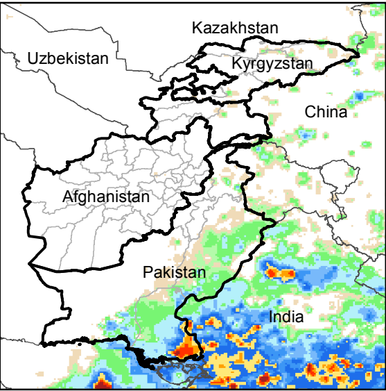
Daily Rainfall estimate for 20 Jul., 2017
