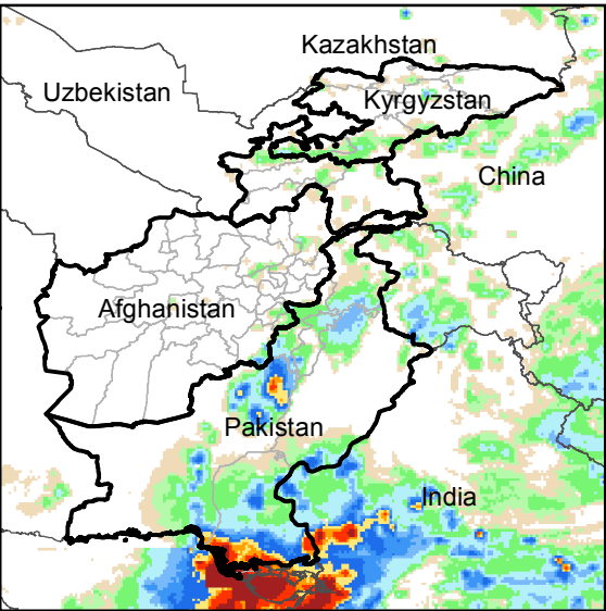
Daily Rainfall estimate for 18 Jul., 2017
