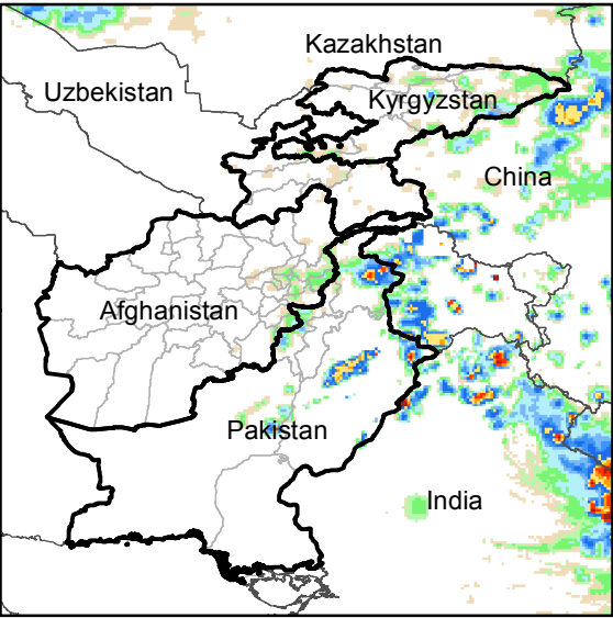
Daily Rainfall estimate for 14 Aug., 2017
