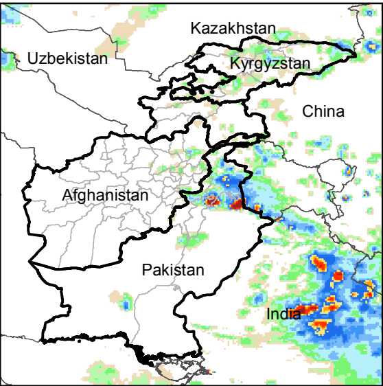
Daily Rainfall estimate for 13 Aug., 2017
