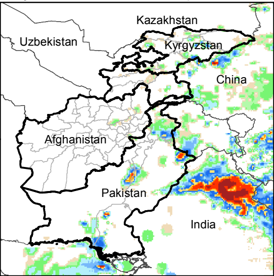
Daily Rainfall estimate for 4 Sep., 2017
