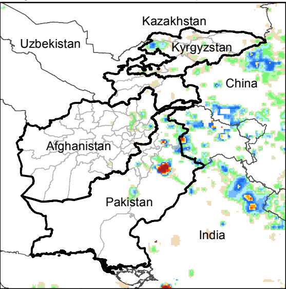
Daily Rainfall estimate for 5 Sep., 2017
