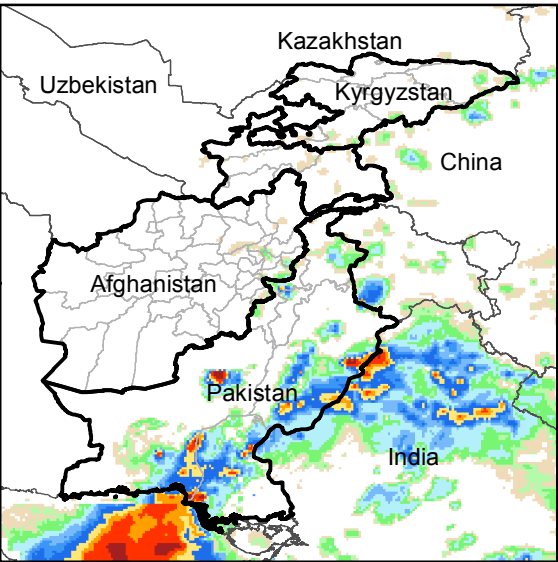
Daily Rainfall estimate for 3 Sep., 2017
