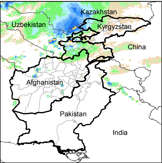
Daily Rainfall estimate for 29 Nov., 2017
