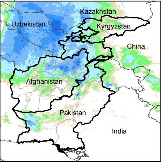
Daily Rainfall estimate for 20 Feb., 2018
