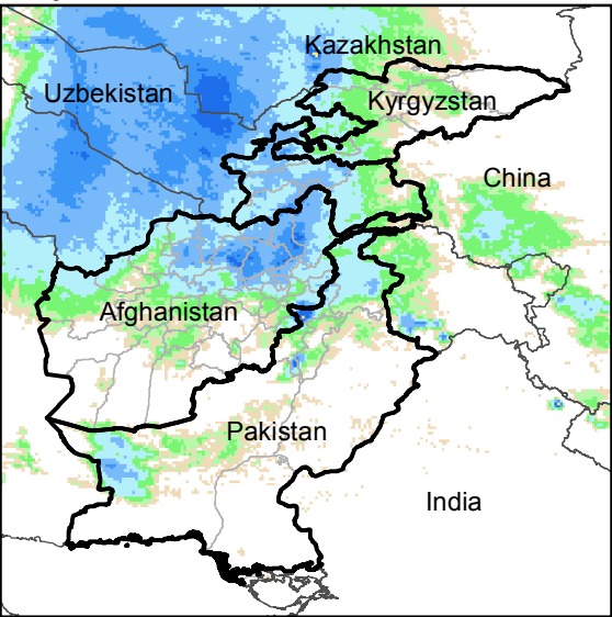
Daily Rainfall estimate for 23 Feb., 2018
