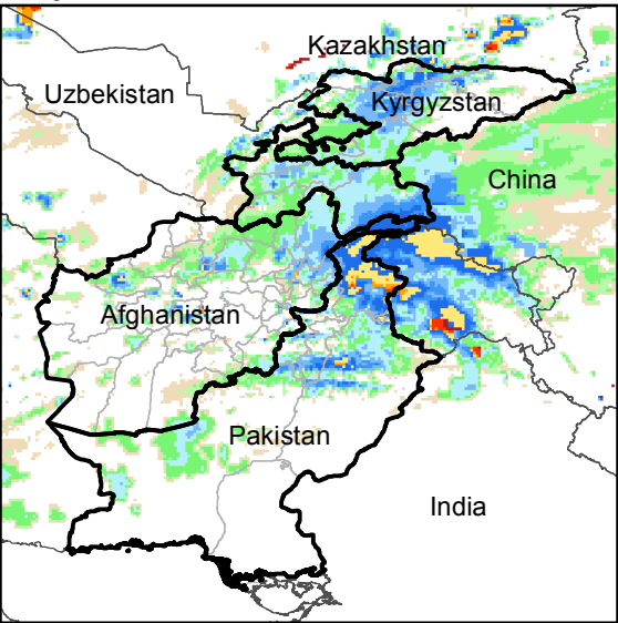
Daily Rainfall estimate for 5 Mar., 2018
