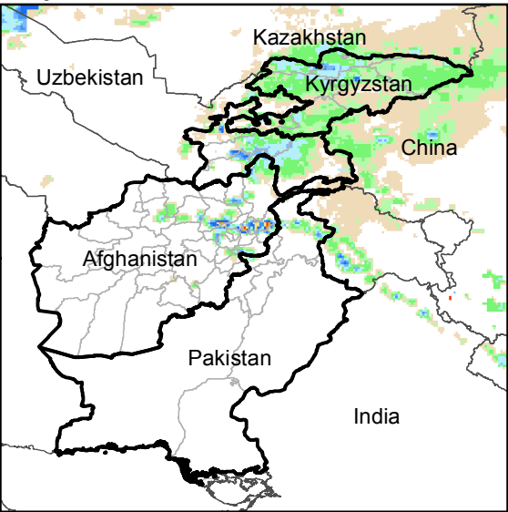
Daily Rainfall estimate for 31 Mar., 2018
