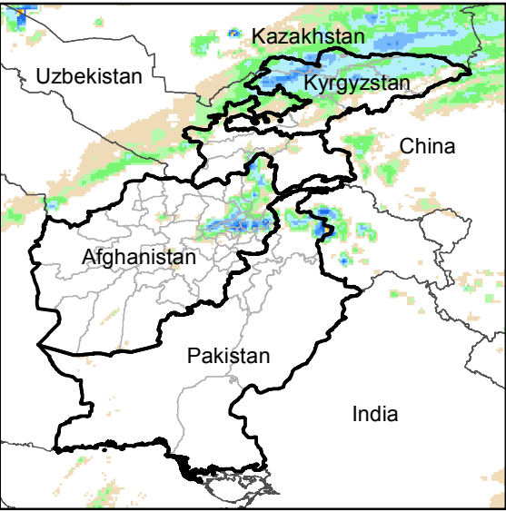
Daily Rainfall estimate for 1 Apr., 2018
