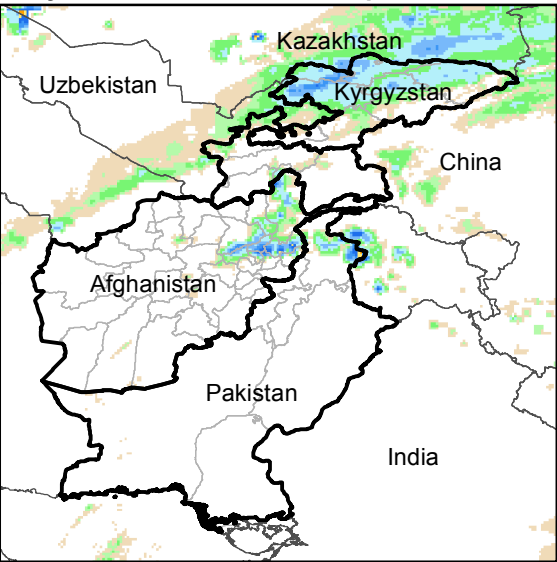
Daily Rainfall estimate for 4 Apr., 2018
