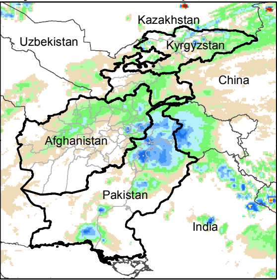
Daily Rainfall estimate for 8 Apr., 2018
