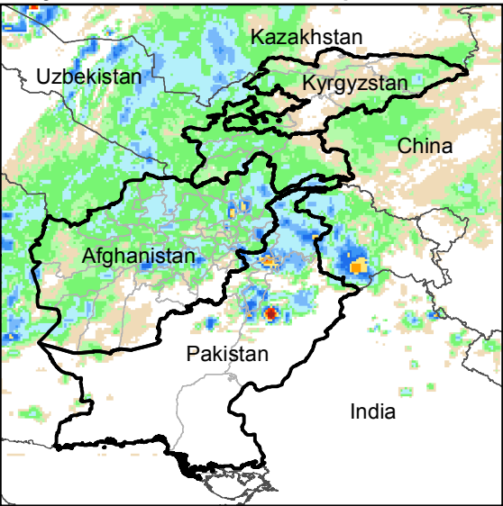
Daily Rainfall estimate for 20 Apr., 2018
