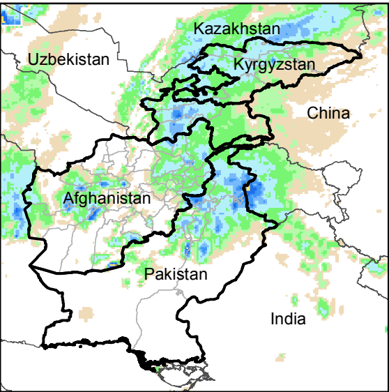
Daily Rainfall estimate for 19 Apr., 2018
