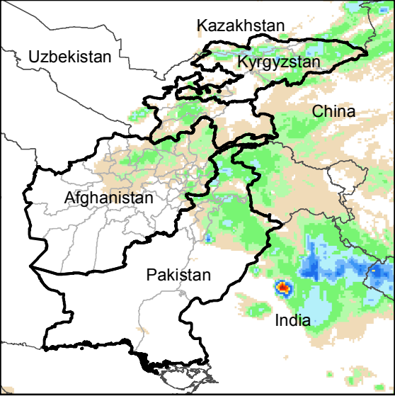
Daily Rainfall estimate for 2 May., 2018
