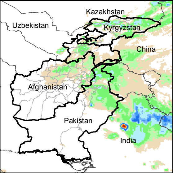
Daily Rainfall estimate for 5 May., 2018
