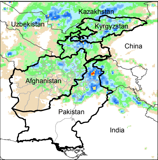
Daily Rainfall estimate for 15 May., 2018
