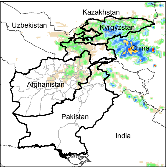
Daily Rainfall estimate for 24 May., 2018
