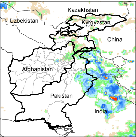
Daily Rainfall estimate for 9 Jun., 2018
