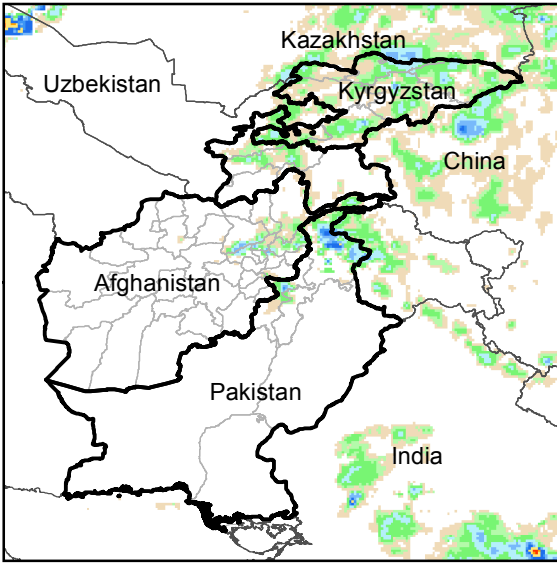
Daily Rainfall estimate for 11 Jun., 2018
