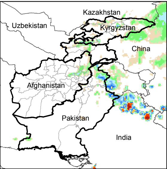
Daily Rainfall estimate for 19 Jun., 2018
