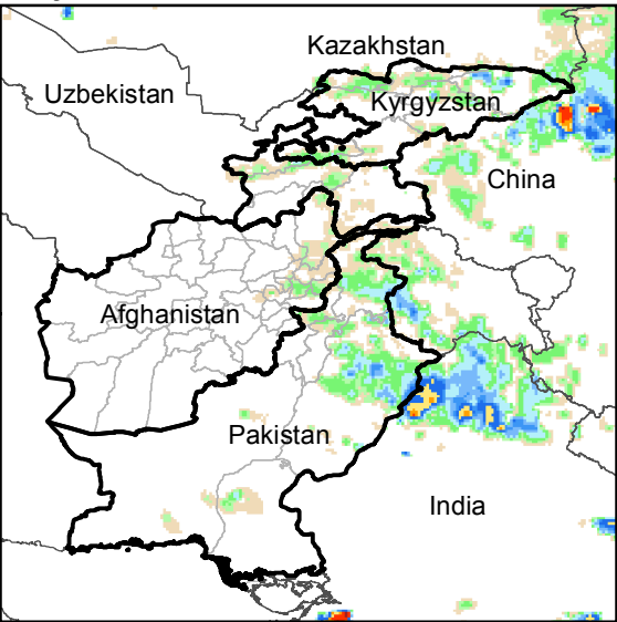
Daily Rainfall estimate for 20 Jun., 2018
