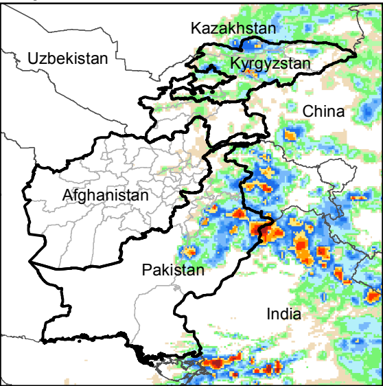
Daily Rainfall estimate for 6 Jul., 2018
