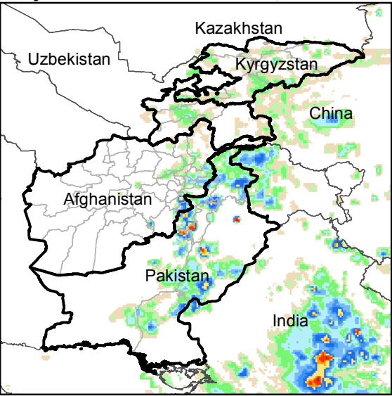
Daily Rainfall estimate for 5 Jul., 2018
