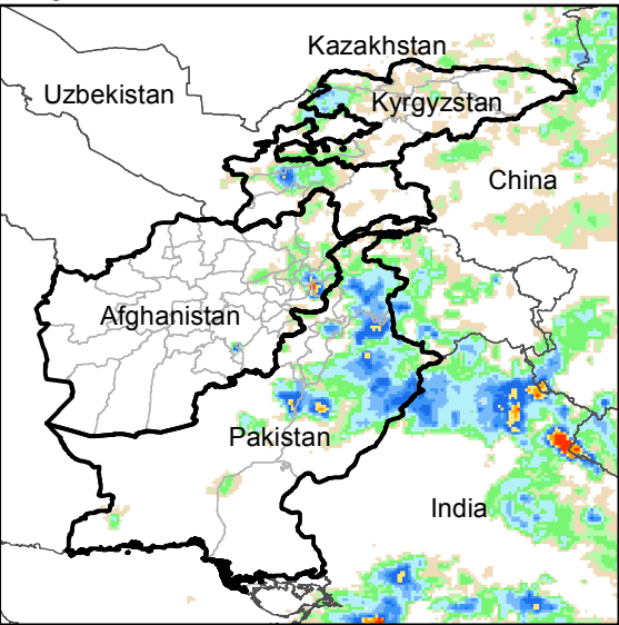
Daily Rainfall estimate for 7 Jul., 2018
