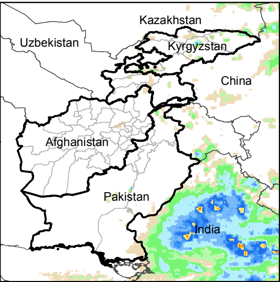
Daily Rainfall estimate for 1 Sep., 2018
