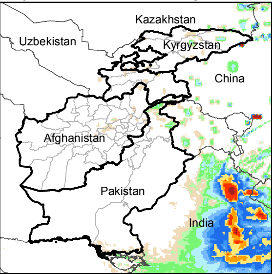
Daily Rainfall estimate for 3 Sep., 2018
