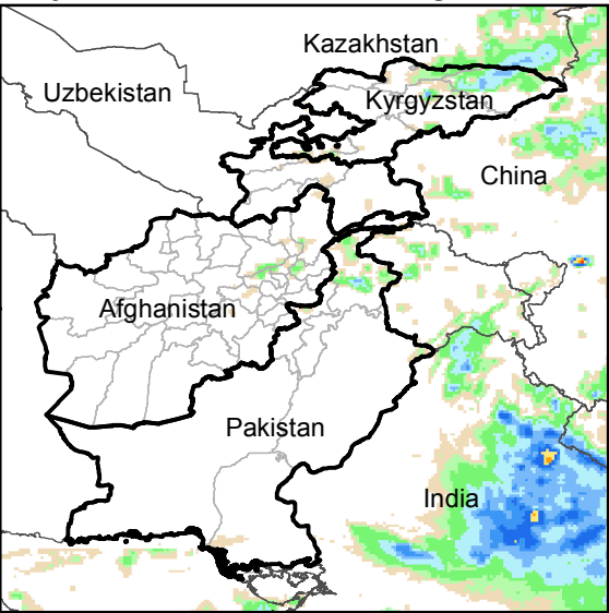
Daily Rainfall estimate for 2 Sep., 2018
