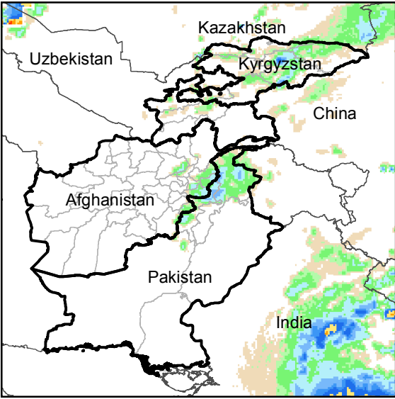
Daily Rainfall estimate for 21 Sep., 2018
