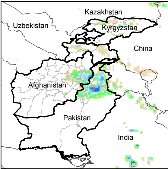
Daily Rainfall estimate for 7 Oct., 2018
