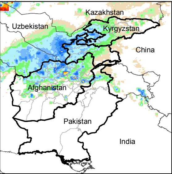
Daily Rainfall estimate for 3 Nov., 2018
