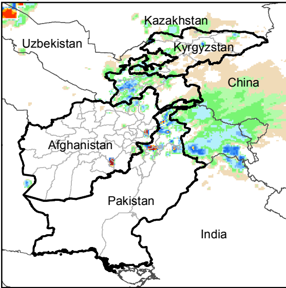
Daily Rainfall estimate for 5 Nov., 2018
