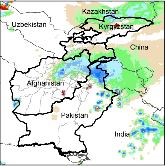
Daily Rainfall estimate for 6 Feb., 2019
