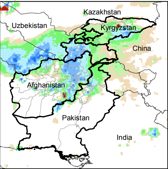
Daily Rainfall estimate for 8 Feb., 2019
