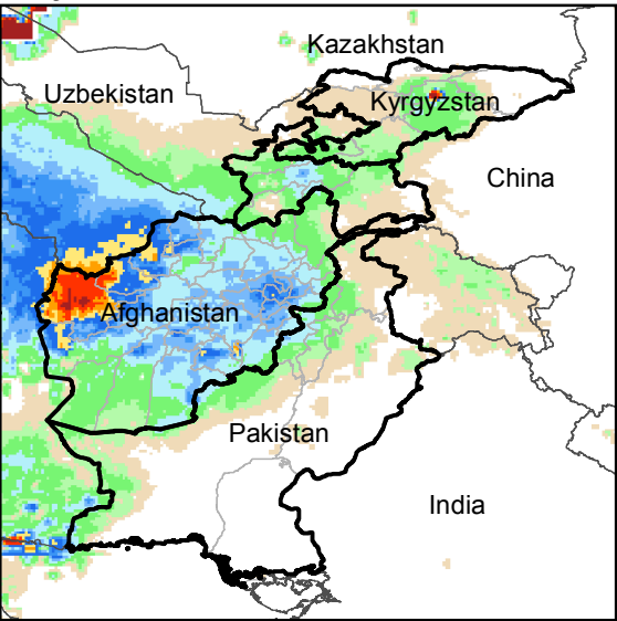
Daily Rainfall estimate for 7 Feb., 2019
