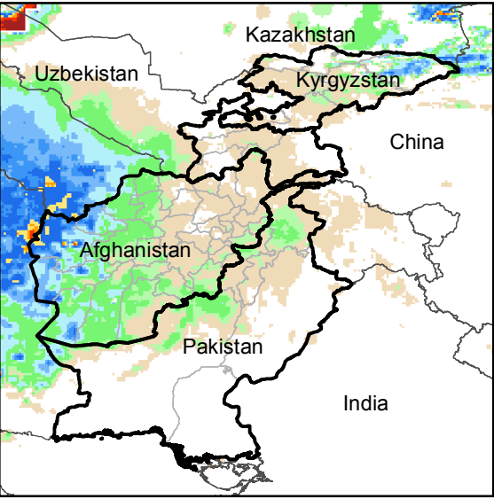
Daily Rainfall estimate for 12 Feb., 2019
