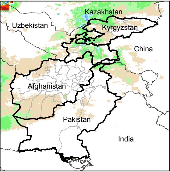
Daily Rainfall estimate for 11 Feb., 2019
