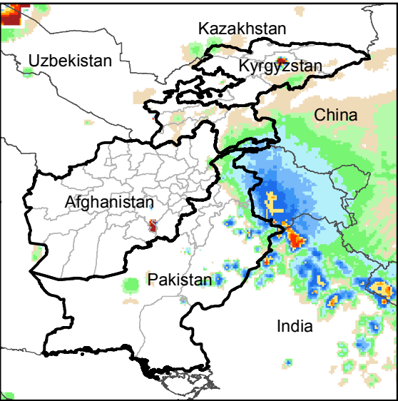
Daily Rainfall estimate for 10 Feb., 2019
