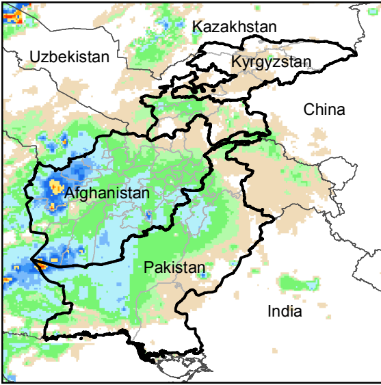
Daily Rainfall estimate for 1 Mar., 2019
