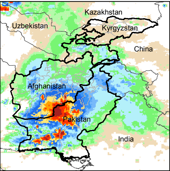
Daily Rainfall estimate for 5 Mar., 2019
