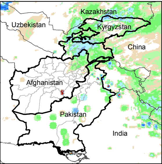
Daily Rainfall estimate for 6 Mar., 2019
