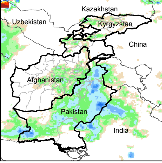
Daily Rainfall estimate for 15 May., 2019
