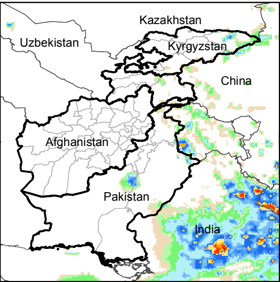
Daily Rainfall estimate for 8 Aug., 2019
