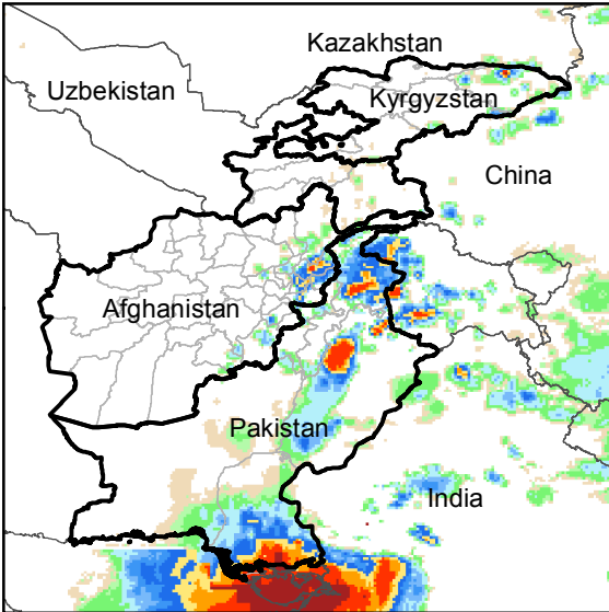
Daily Rainfall estimate for 10 Aug., 2019
