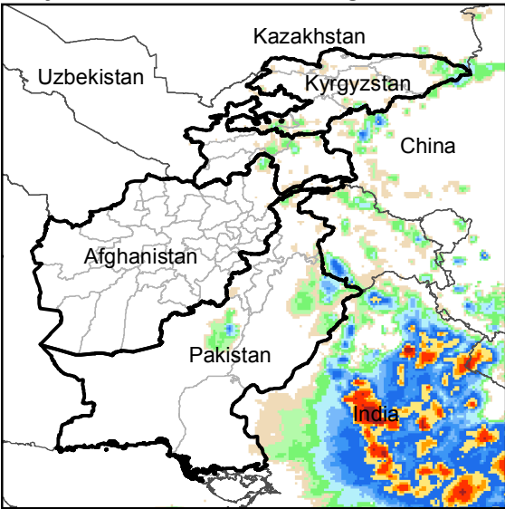
Daily Rainfall estimate for 9 Aug., 2019
