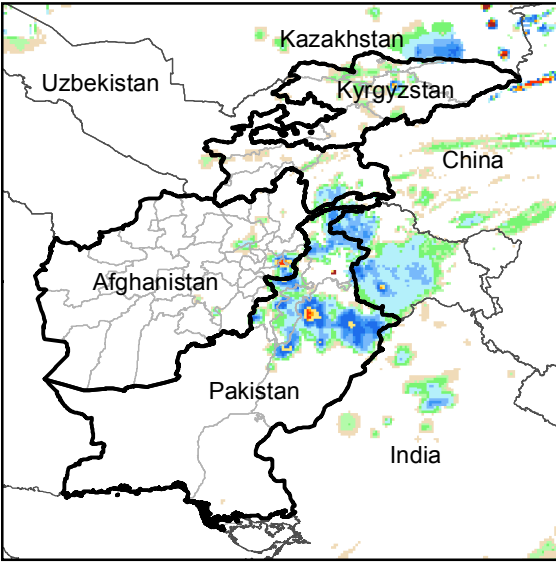
Daily Rainfall estimate for 18 Oct., 2019
