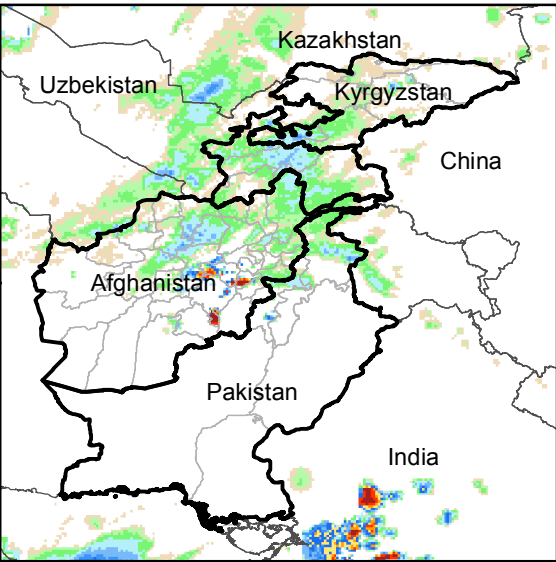
Daily Rainfall estimate for 2 Nov., 2019
