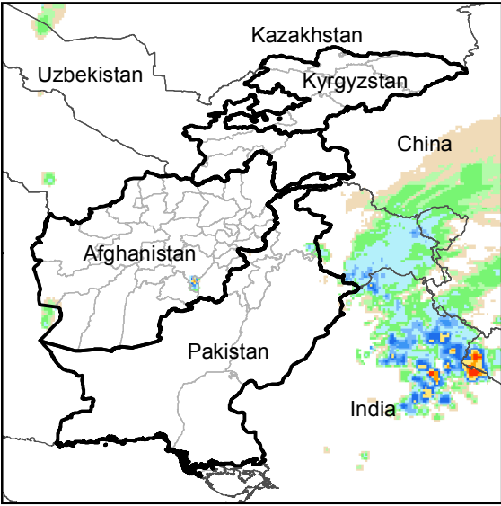
Daily Rainfall estimate for 28 Nov., 2019
