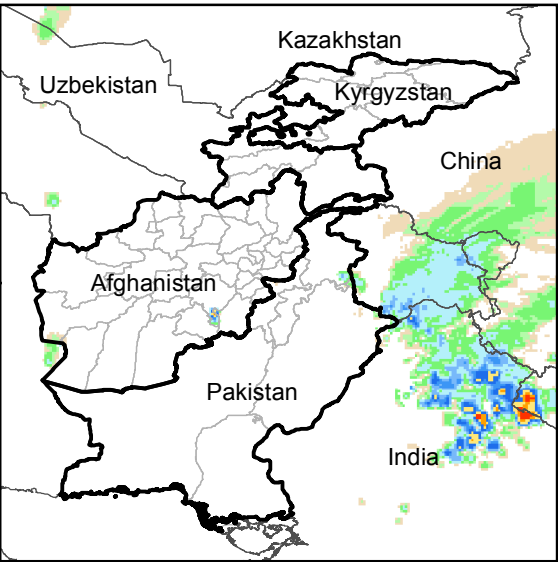
Daily Rainfall estimate for 1 Dec., 2019
