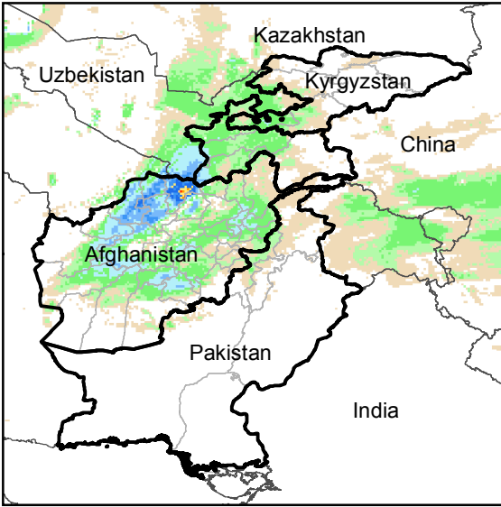
Daily Rainfall estimate for 10 Dec., 2019
