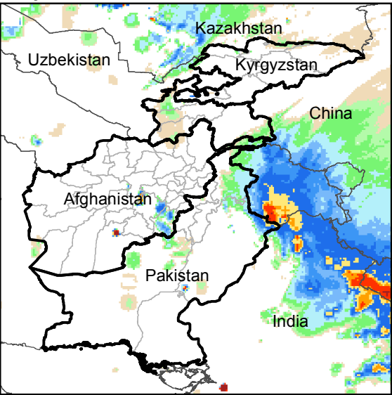
Daily Rainfall estimate for 16 Dec., 2019
