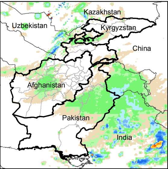
Daily Rainfall estimate for 15 Dec., 2019
