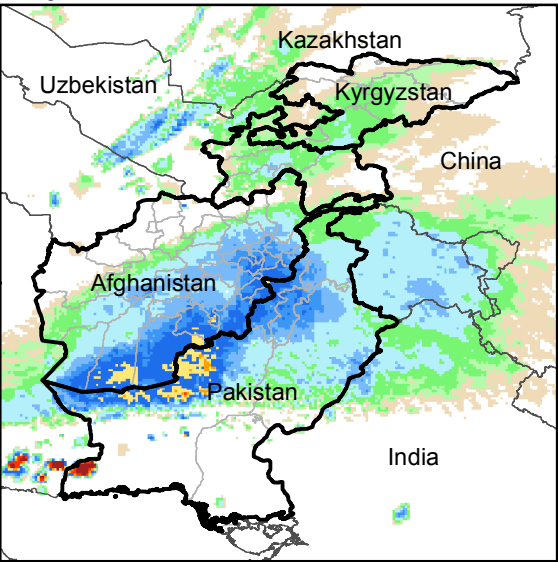
Daily Rainfall estimate for 9 Jan., 2020
