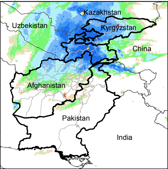
Daily Rainfall estimate for 6 Feb., 2020
