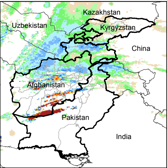
Daily Rainfall estimate for 15 Feb., 2020
