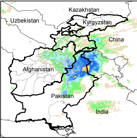
Daily Rainfall estimate for 28 Feb., 2020
