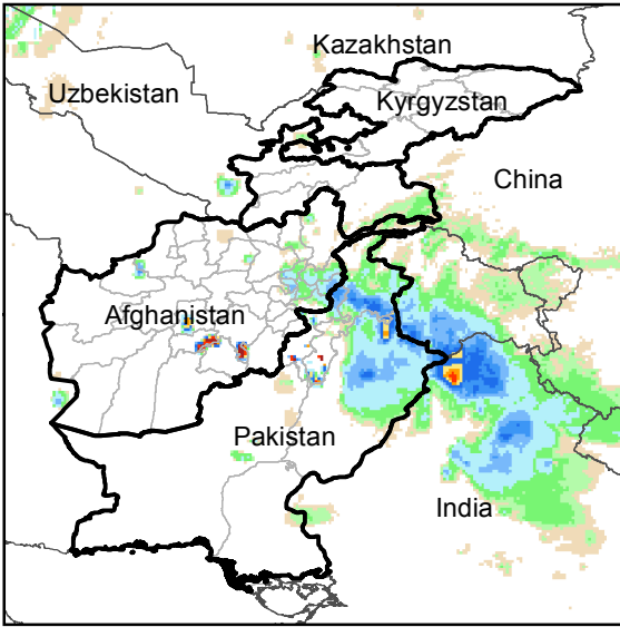
Daily Rainfall estimate for 29 Feb., 2020
