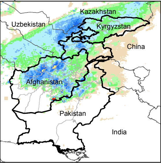
Daily Rainfall estimate for 27 Feb., 2020
