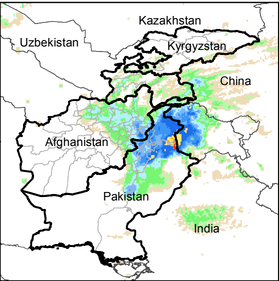
Daily Rainfall estimate for 2 Mar., 2020
