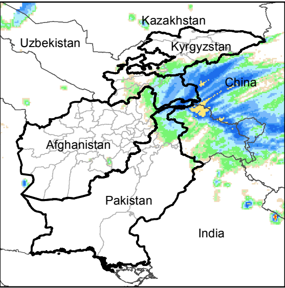
Daily Rainfall estimate for 7 Mar., 2020
