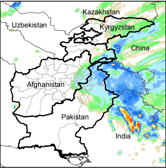
Daily Rainfall estimate for 6 Mar., 2020
