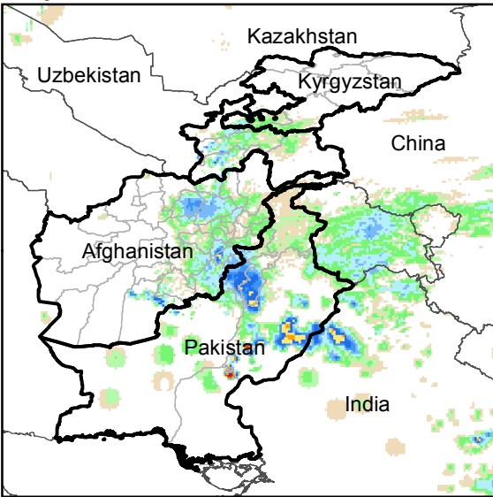
Daily Rainfall estimate for 14 Mar., 2020
