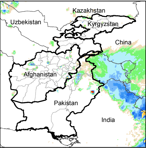
Daily Rainfall estimate for 13 Mar., 2020
