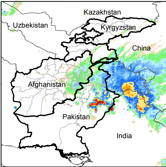
Daily Rainfall estimate for 15 Mar., 2020
