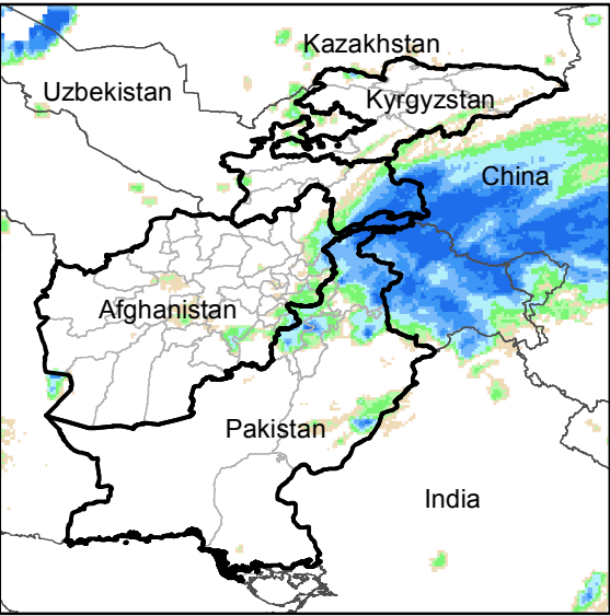
Daily Rainfall estimate for 28 Mar., 2020
