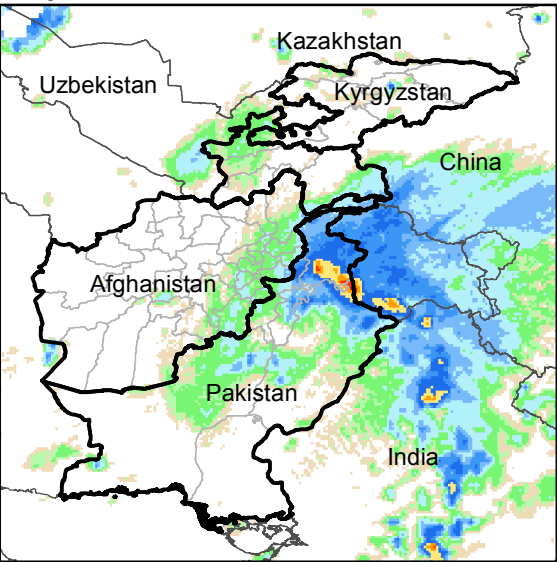
Daily Rainfall estimate for 30 Mar., 2020
