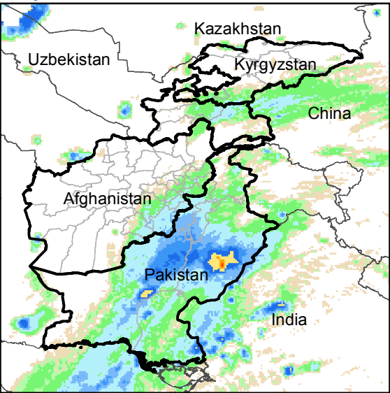
Daily Rainfall estimate for 29 Mar., 2020
