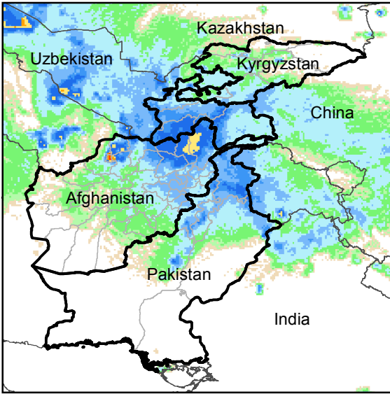
Daily Rainfall estimate for 31 Mar., 2020
