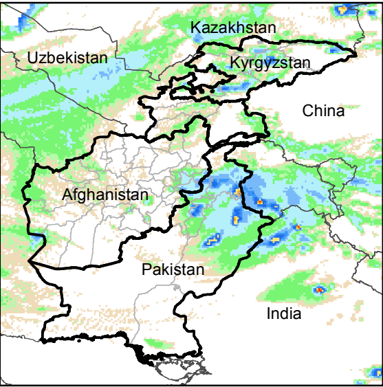
Daily Rainfall estimate for 7 Apr., 2020
