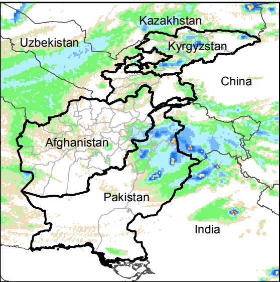
Daily Rainfall estimate for 10 Apr., 2020
