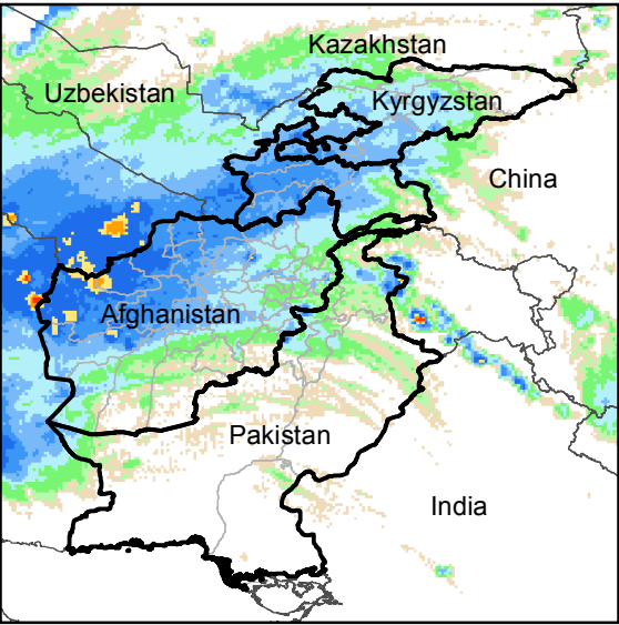
Daily Rainfall estimate for 11 Apr., 2020
