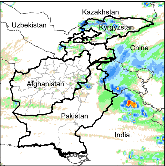
Daily Rainfall estimate for 21 Apr., 2020
