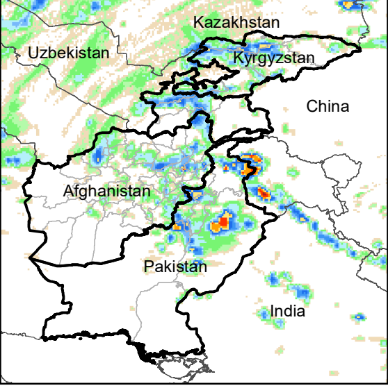
Daily Rainfall estimate for 24 Apr., 2020
